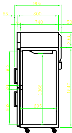
SIDE VIEW (Half Glass Door)
