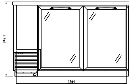
TBB-2SG FRONT VIEW
