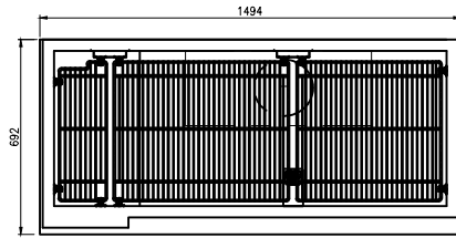
PLAN VIEW (TBB-2SB/SG)
