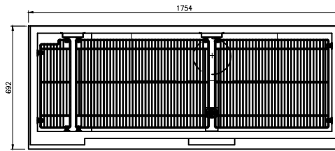
PLAN VIEW (TBB-3SB/SG)
