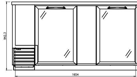
TBB-3SG FRONT VIEW
