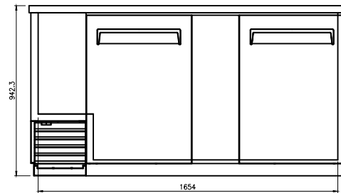
TBB-3SB FRONT VIEW
